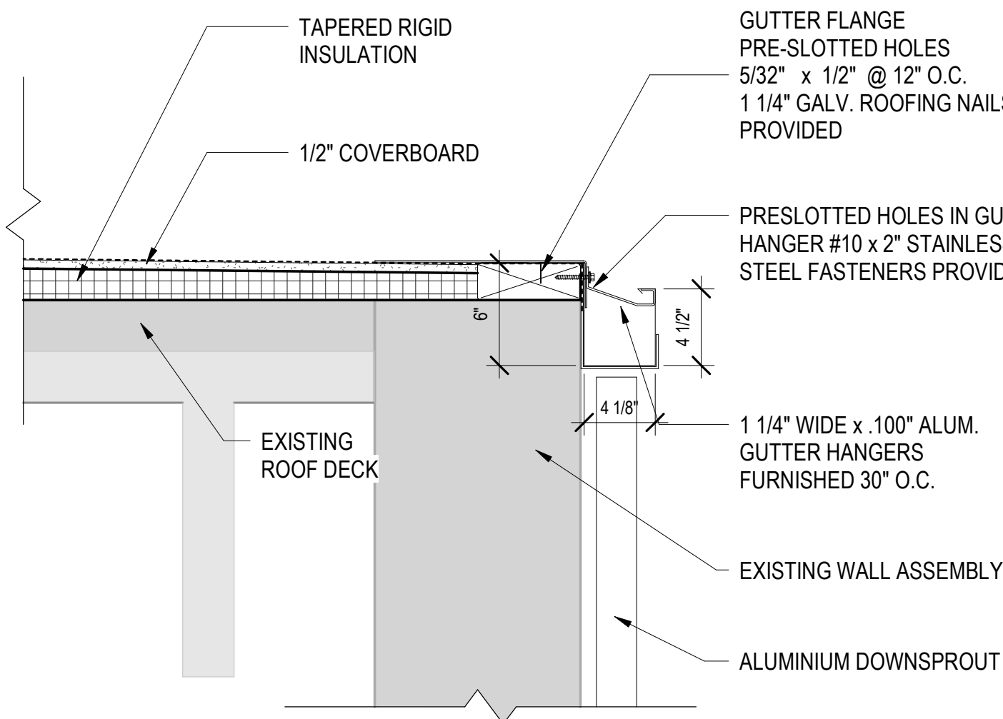
2 DETAIL @ ROOF GUTTER 1 1/2" = 1'-0"
