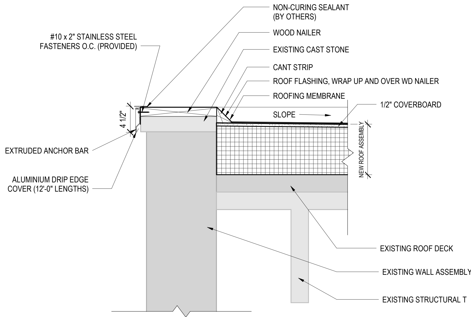
1 DETAIL @ ROOF 1 1/2" = 1'-0"
