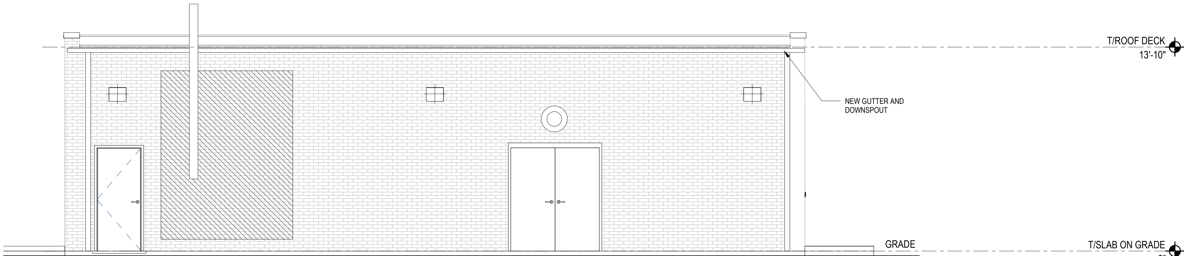
3 SOUTH ELEVATION 1/4" = 1'-0"
