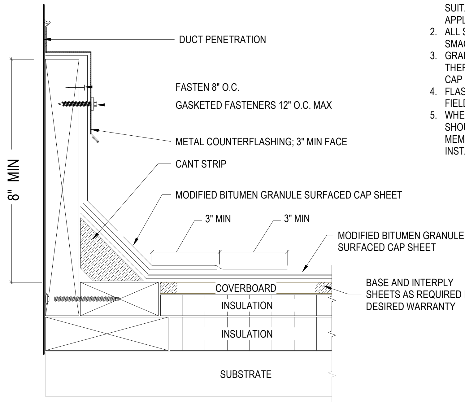
6 DETAIL @ ROOF PENETRATION N.T.S.
