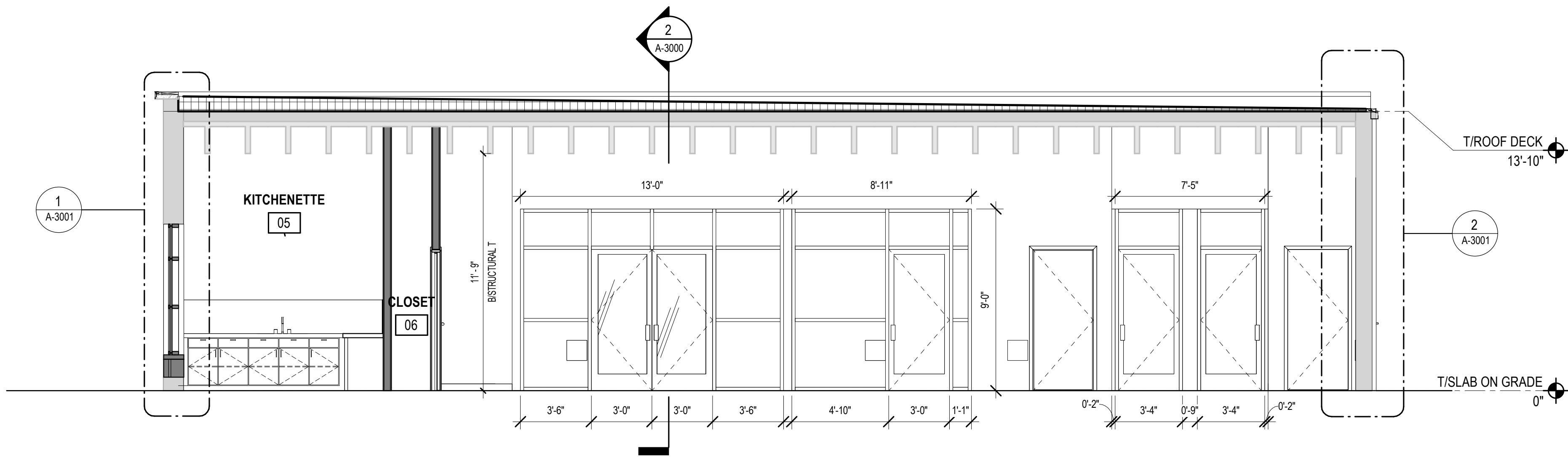
1 NORTH-SOUTH SECTION 1/4" = 1'-0"
